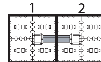
B SE00268 45mm interconnection Lead
